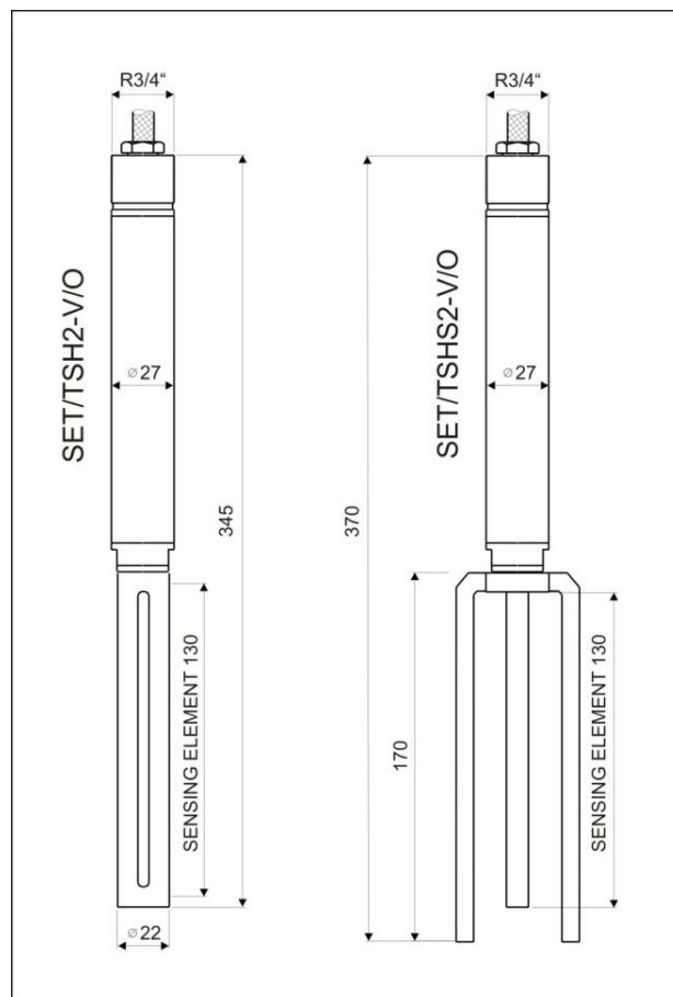
Fig. 1. SET/TSH2 and SET/TSHS2 dimensional drawings
