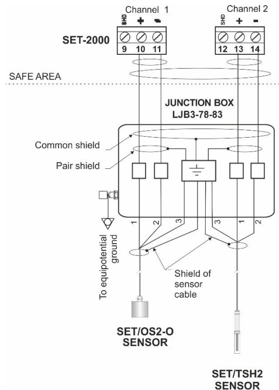
Figure 4. Level sensor cabling with a junction box when the level sensors are in same area and same zone.
