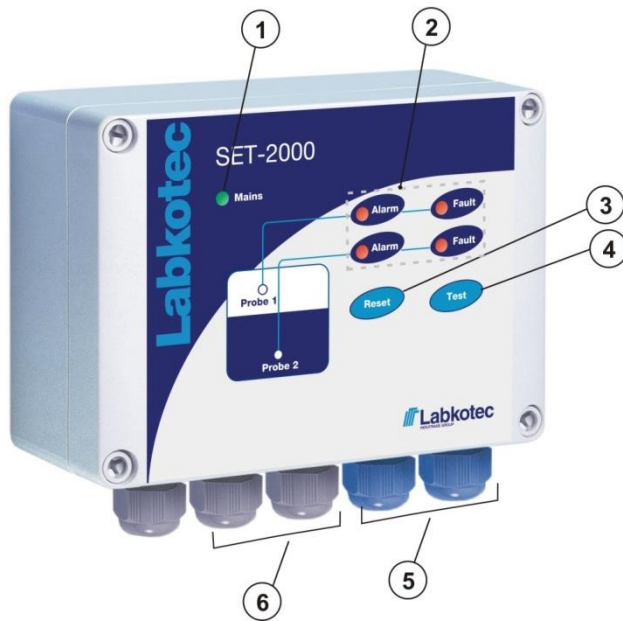
Figure 1. SET-2000 level switch – features
