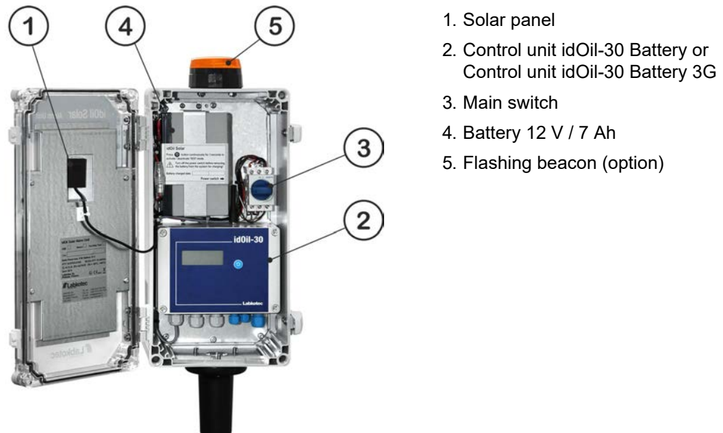
Figure 2. System components - idOil Solar Control unit
