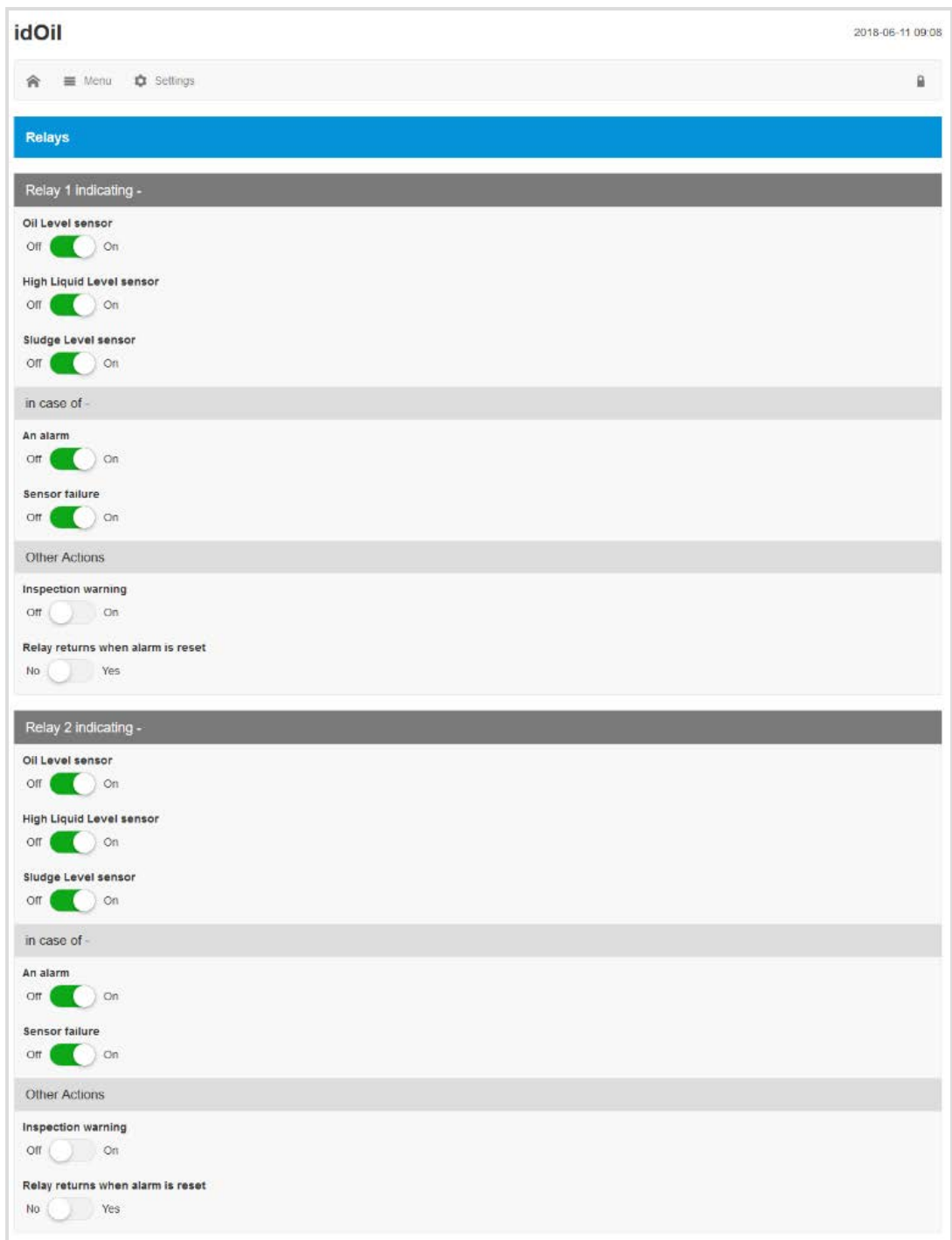
Figure 39. Relay settings
